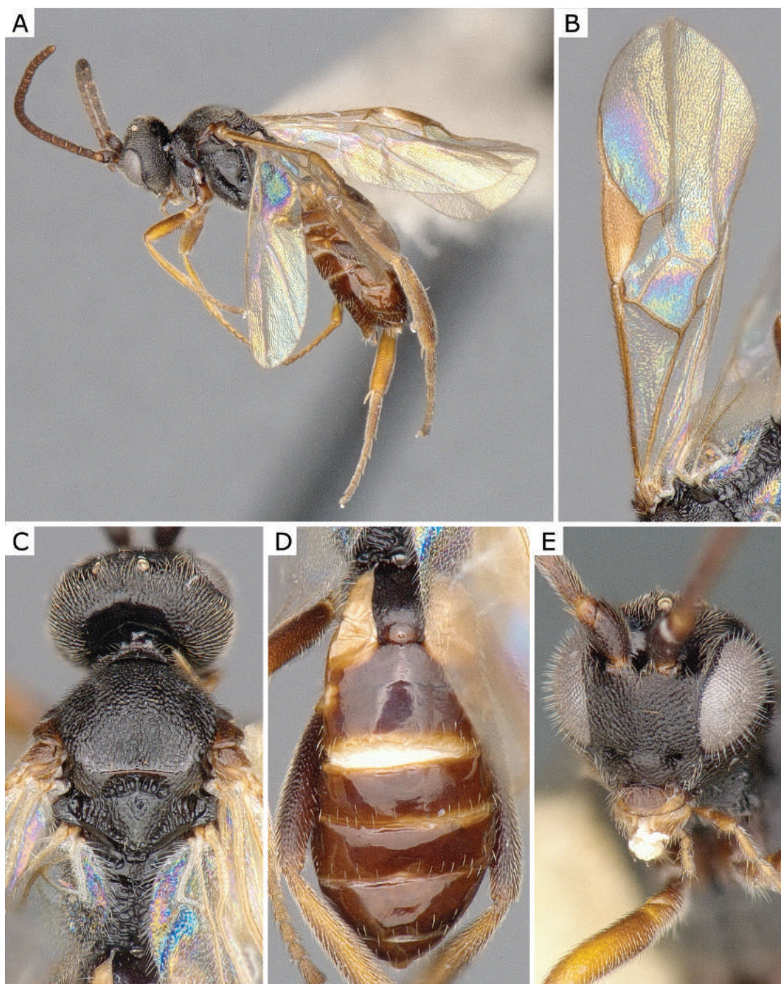
Figure 39. Microplitis coactus (Lundbeck, 1896), female (CNC497575) A lateral view B forewing C mesosoma D metasoma E head frontal view.
