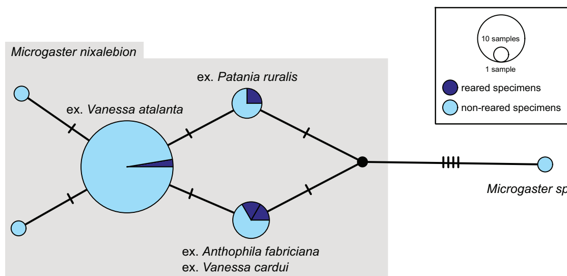
Figure 34. TCS haplotype network of BIN BOLD:ABY6385 , sequence length for analysis: 392 bp to accommodate MRS_JFT0342=MARKB109-21 ex. Anthophila fabriciana from the United Kingdom. The haplotypes morphologically identified as Microgaster nixalebion as part of this project are marked by a grey background. Each hatch mark in the network represents a single mutational change; small black dots at nodes indicate missing haplotypes. The diameter of the circles is proportional to the number of haplotypes sampled (see legend). The aligned sequences and traits can be reviewed in Suppl. materials 10, 11.
