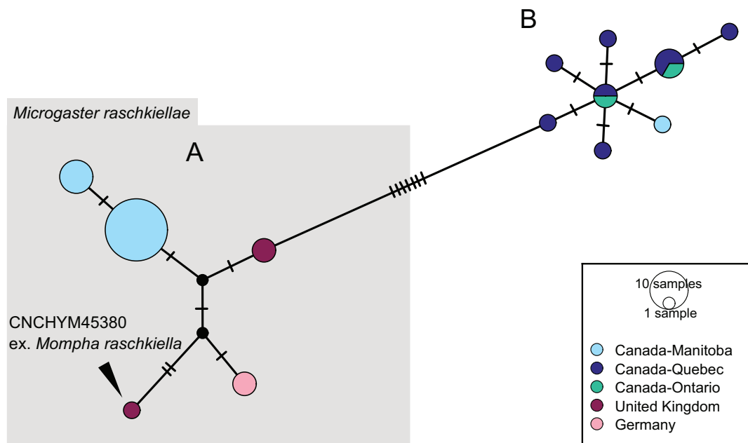
Figure 36. TCS haplotype network of BIN BOLD:AAC9130 , the haplotypes morphologically identified as Microgaster raschkiellae as part of this project are in cluster A and marked by a grey background. Each hatch mark in the network represents a single mutational change; small black dots at nodes indicate missing haplotypes. The diameter of the circles is proportional to the number of haplotypes sampled (see legend). The aligned sequences and traits can be reviewed in Suppl. materials 12, 13.
