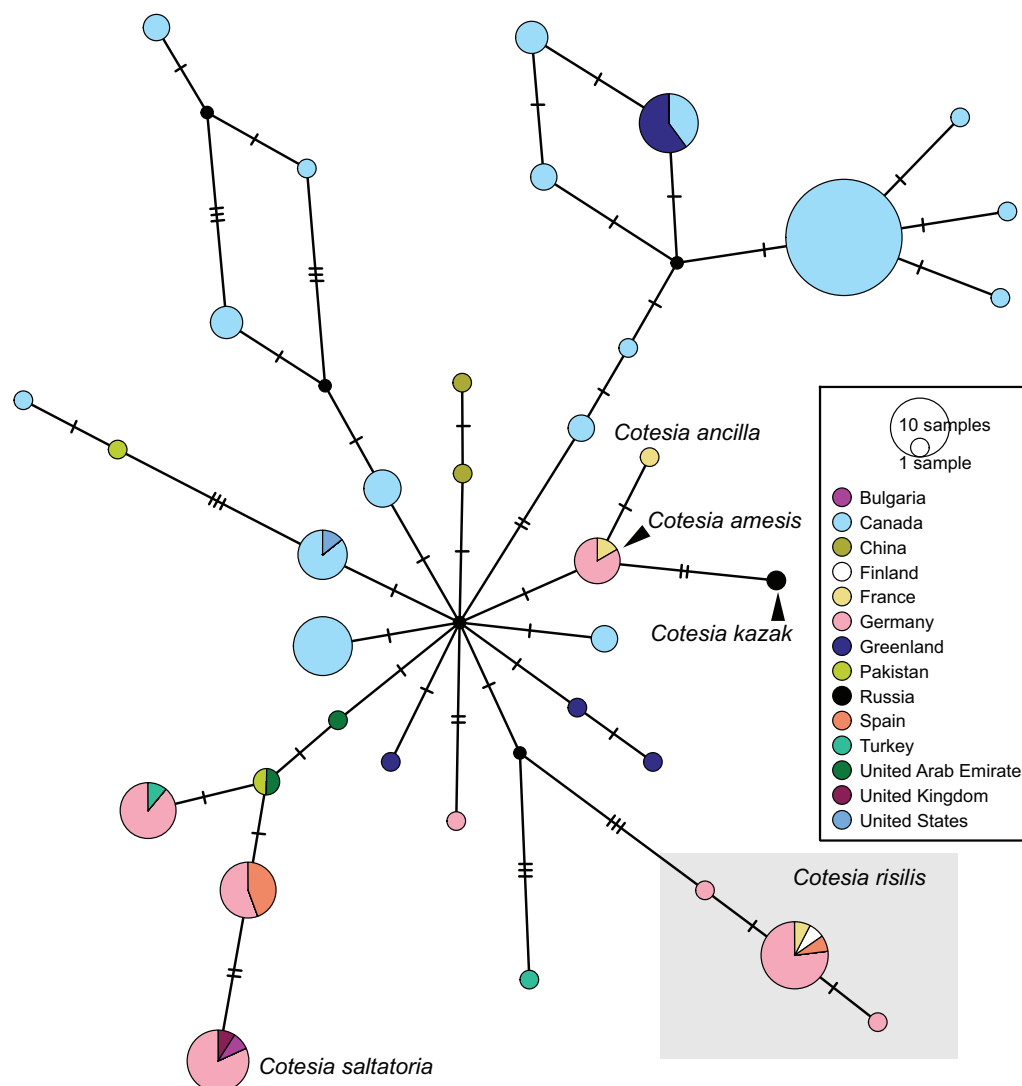
Figure 14. TCS haplotype network of BIN BOLD:AAA6099 , sequence length for analysis: 504 bp. The haplotypes morphologically identified as Cotesia risilis as part of this project are marked by a box. Each hatch mark in the network represents a single mutational change; small black dots at nodes indicate missing haplotypes. The diameter of the circles is proportional to the number of haplotypes sampled and the countries are colour-coded. The aligned sequences and traits can be reviewed in Suppl. materials 8, 9.
